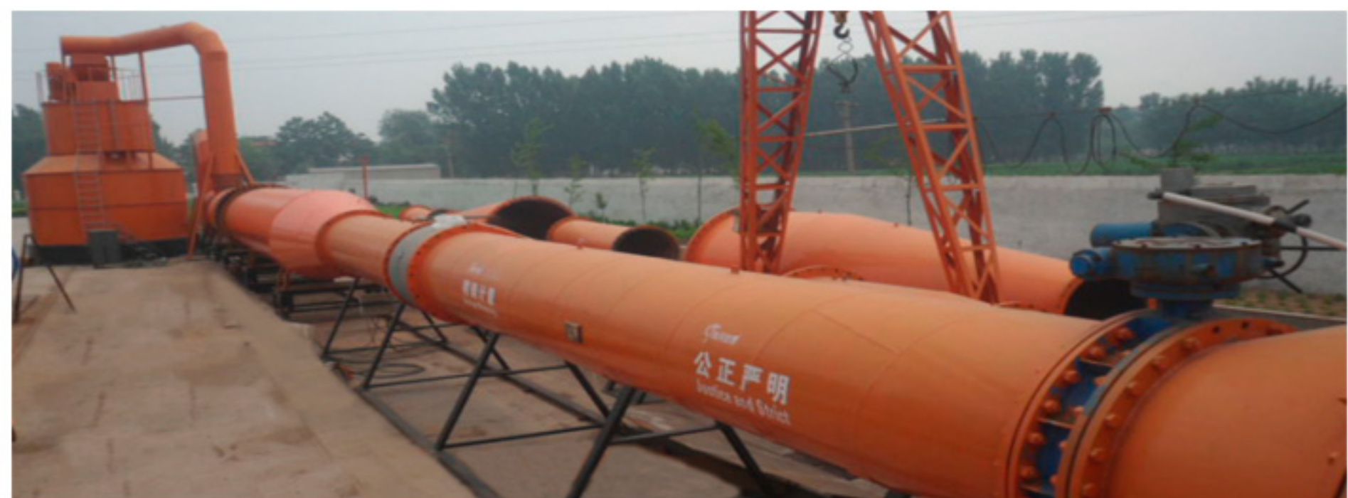
DN800 ~DN3000 Liquid Flow Meter Calibration Device
